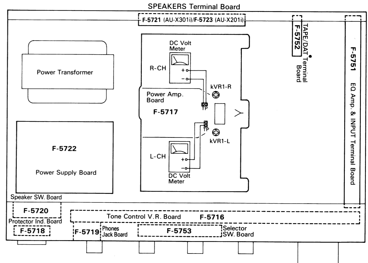
Fig. 5-1 Printed Circuit Location and adjustment points.
