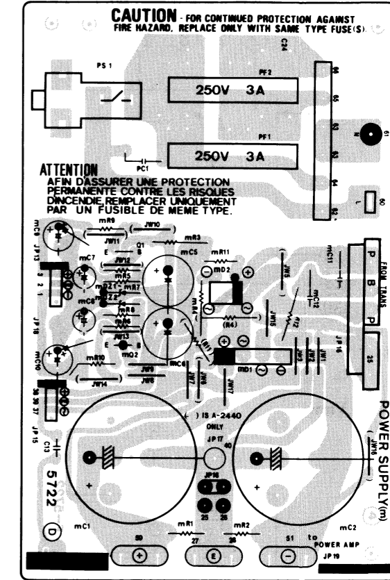
3-9. F-5722 Power Supply Board
